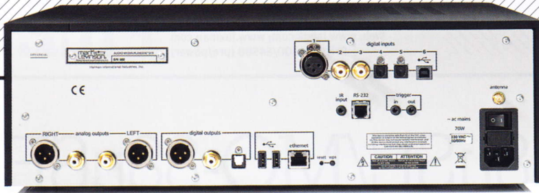
ABOVE: Two coaxial/optical S/PDIF digital ins are joined by USB 2.0 and AES/EBU ins, two USB-A sockets and wired/wireless Ethernet. Coaxial/optical and AES digital outputs are included alongside single-ended (RCA) and balanced (XLR) analogue outs
